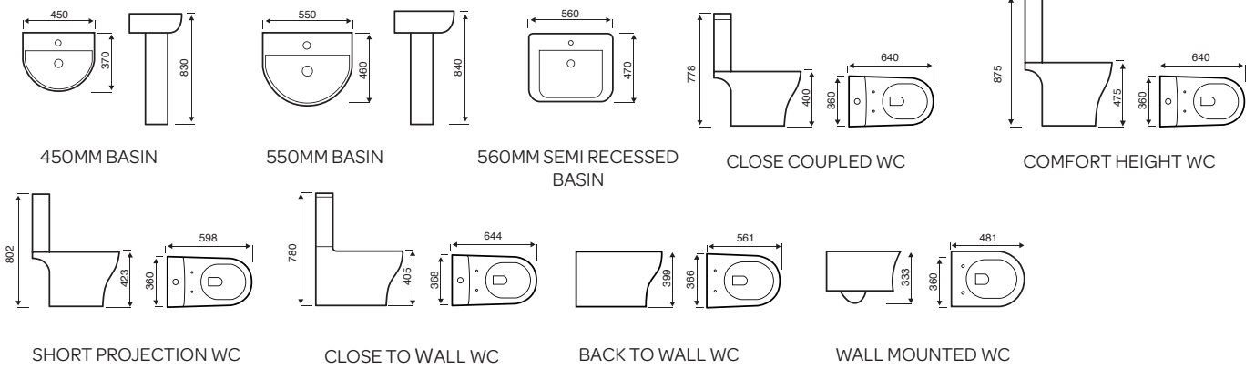
SHORT PROJECTION WC
